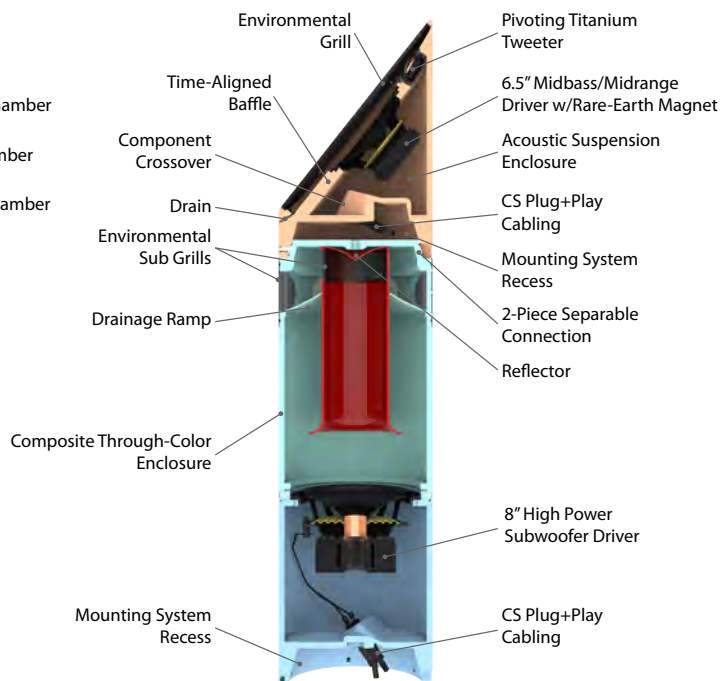
CROSS SECTION OF THE PATENTED 3-WAY ELLIPSE BOLLARD
